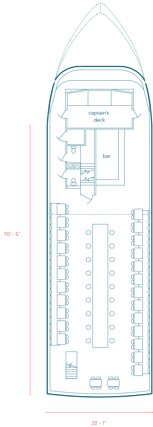
EXTERIOR TOPSIDE DECK
